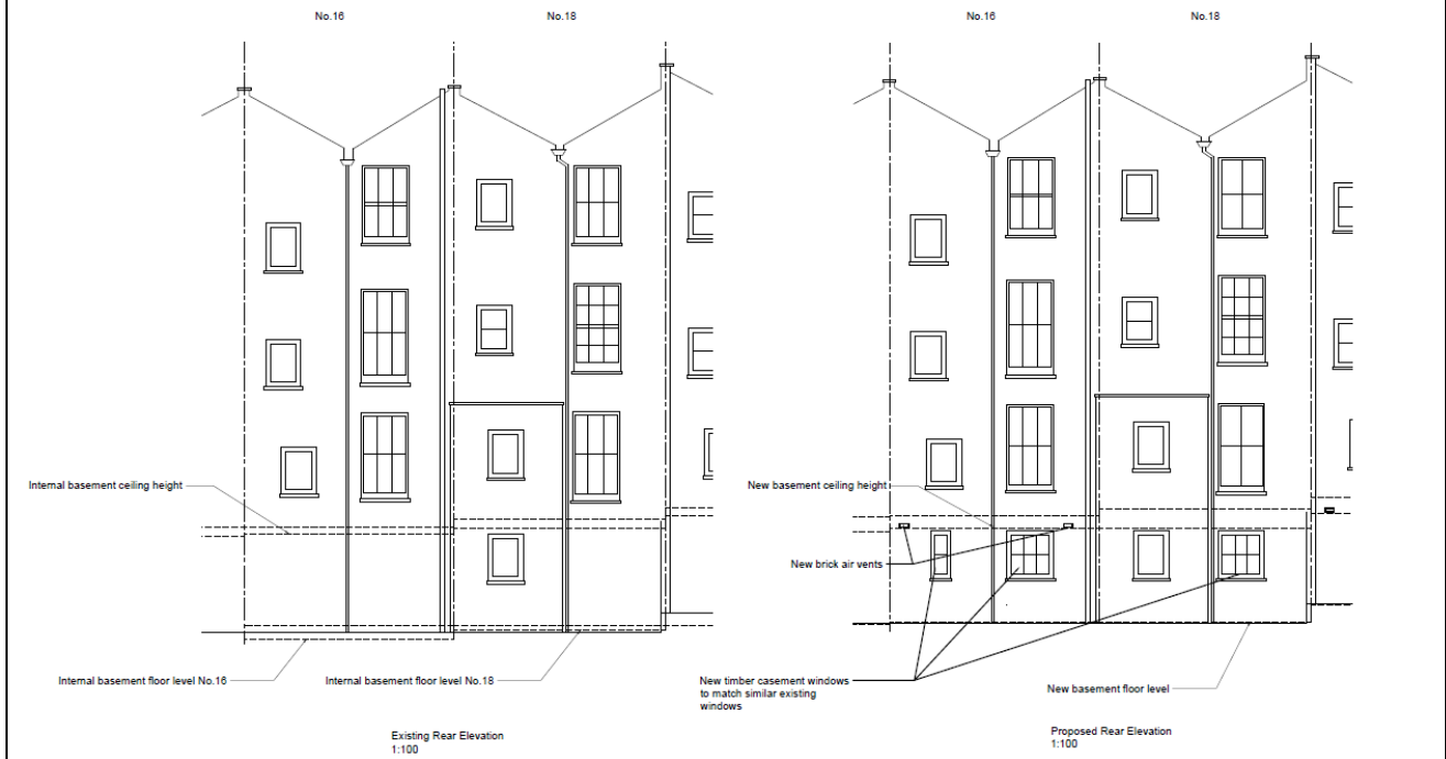
Existing and proposed rear elevations.
